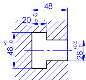
T-slot Section
