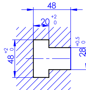
T-slot Section
