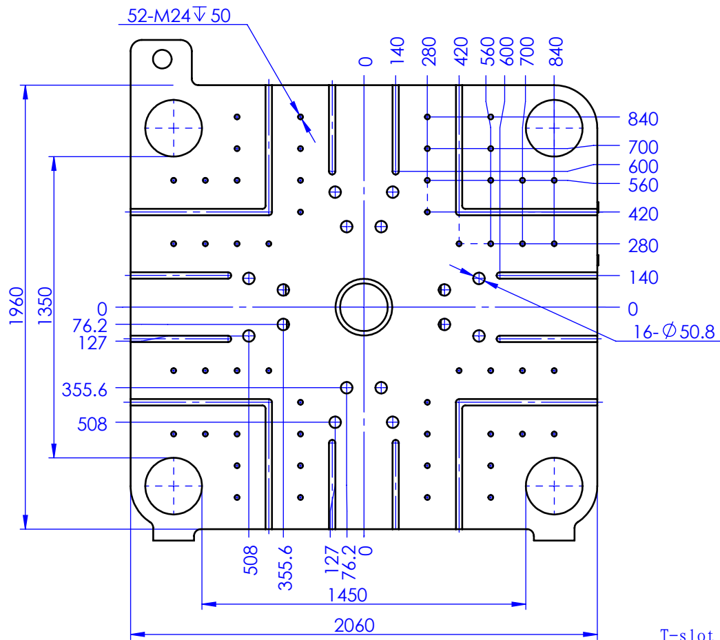
T-slot Section
