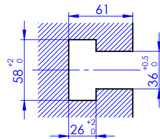
T-Slot Section
