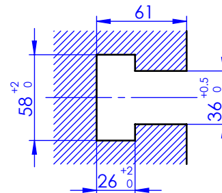
T-Slot Section
